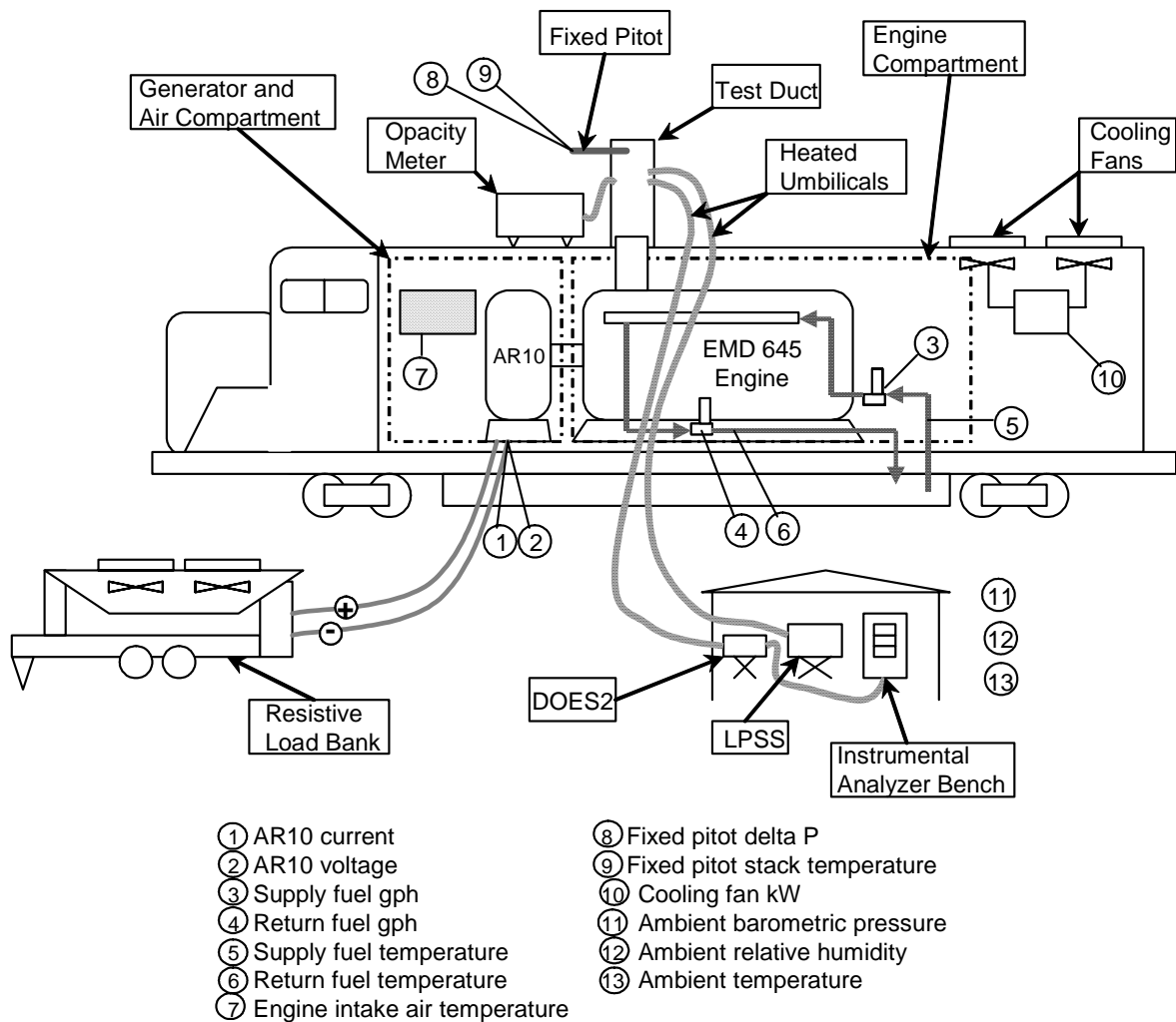
Figure 1-3. Measurement Equipment Locations
