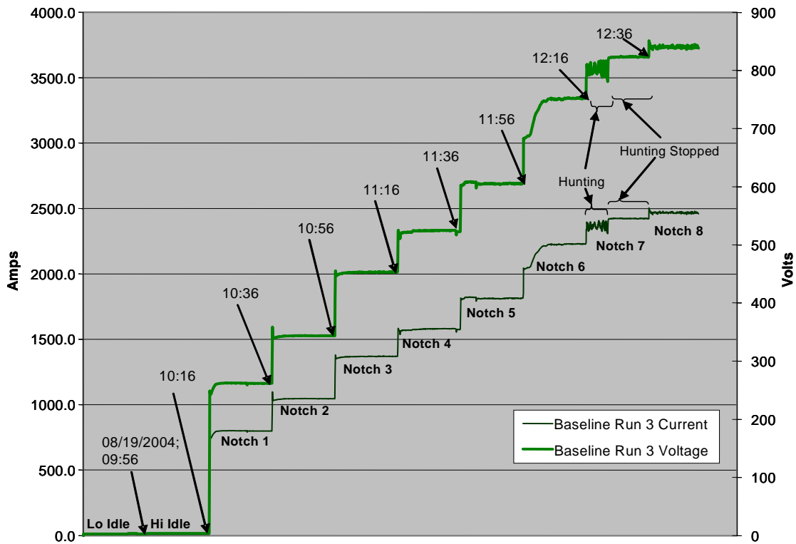
Figure 2-1. AR10 Generator Performance
