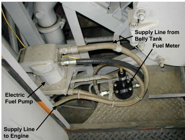
Figure 1-4. Supply Flowmeter
