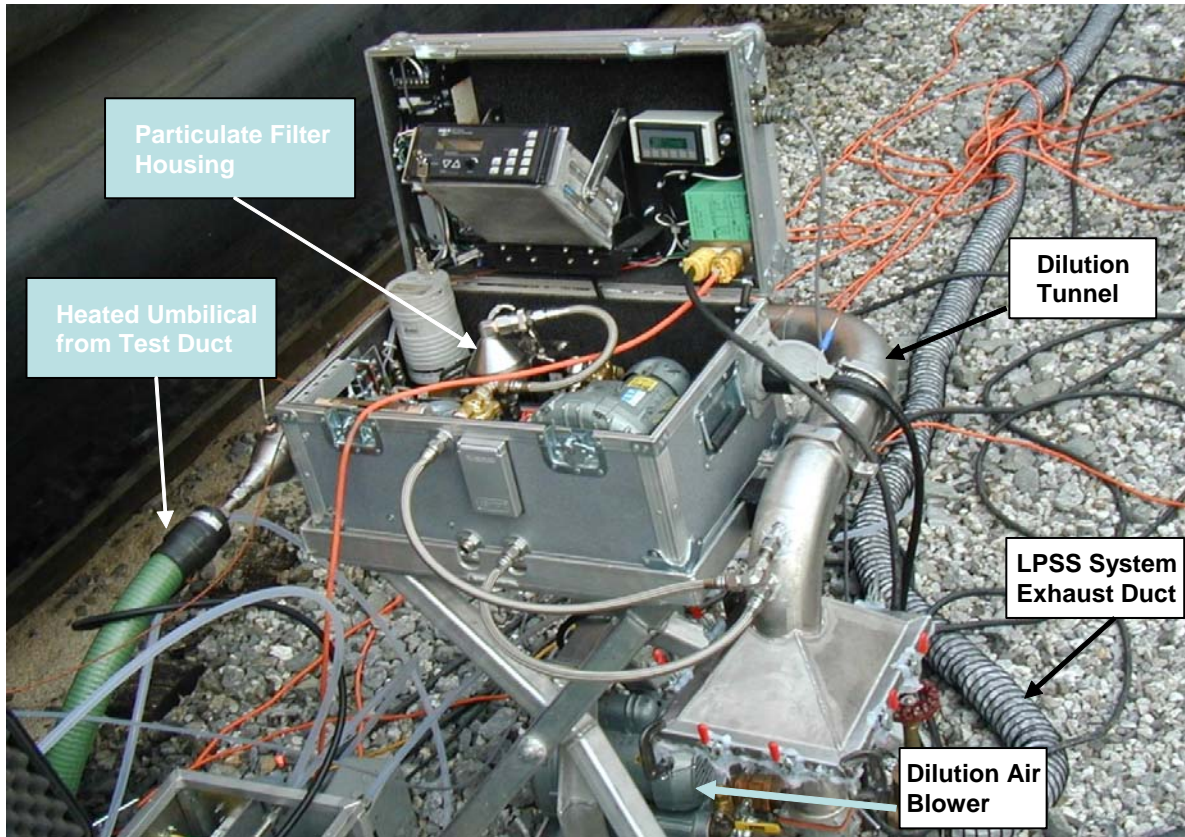
Figure 1-7. Locomotive Particulate Sampling System
