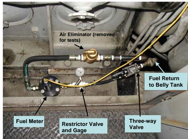
Figure 1-5. Return Flowmeter
